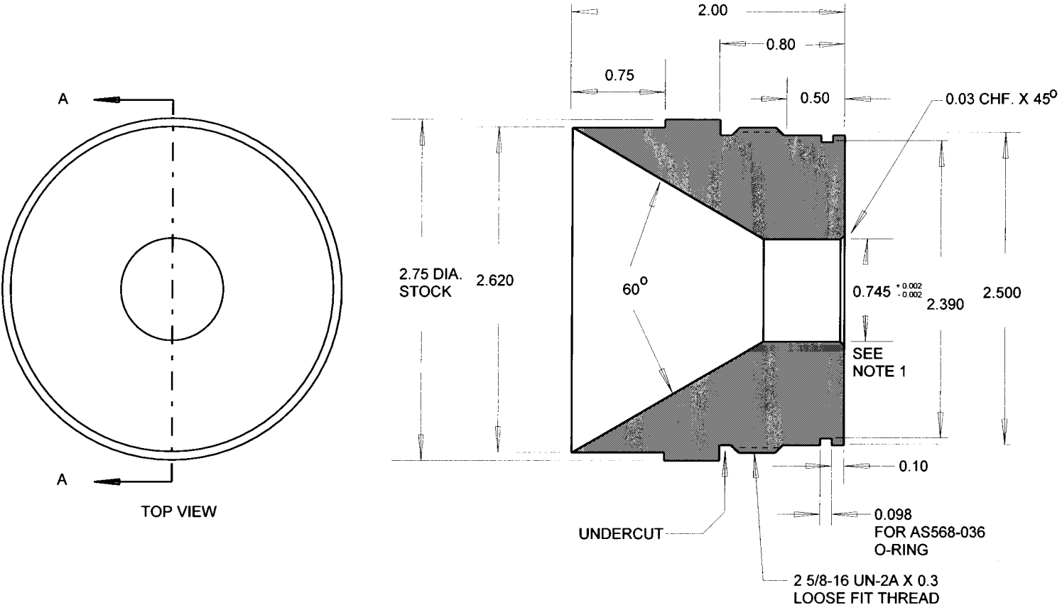
FIGURE L-13. 10-MICRON IMPACTOR NOZZLE
